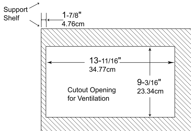
MC2102 Bottom View in Custom Cabinet
