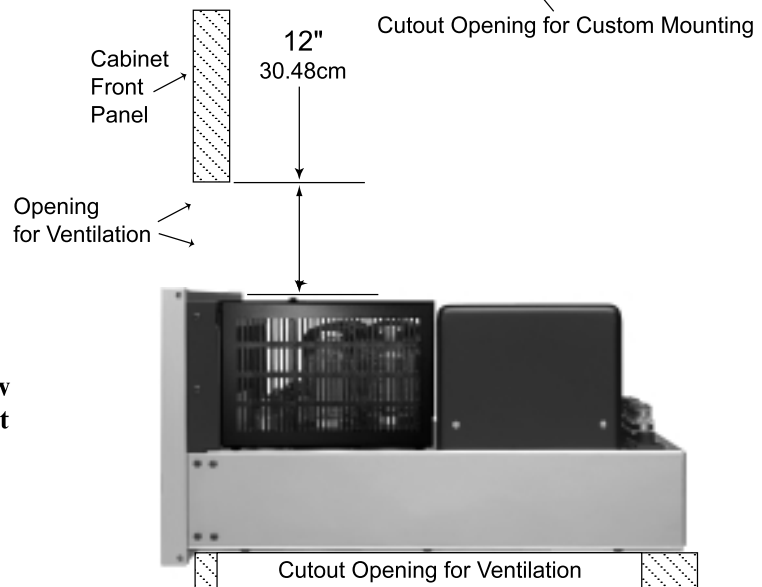
MC2102 Side View in Custom Cabinet
